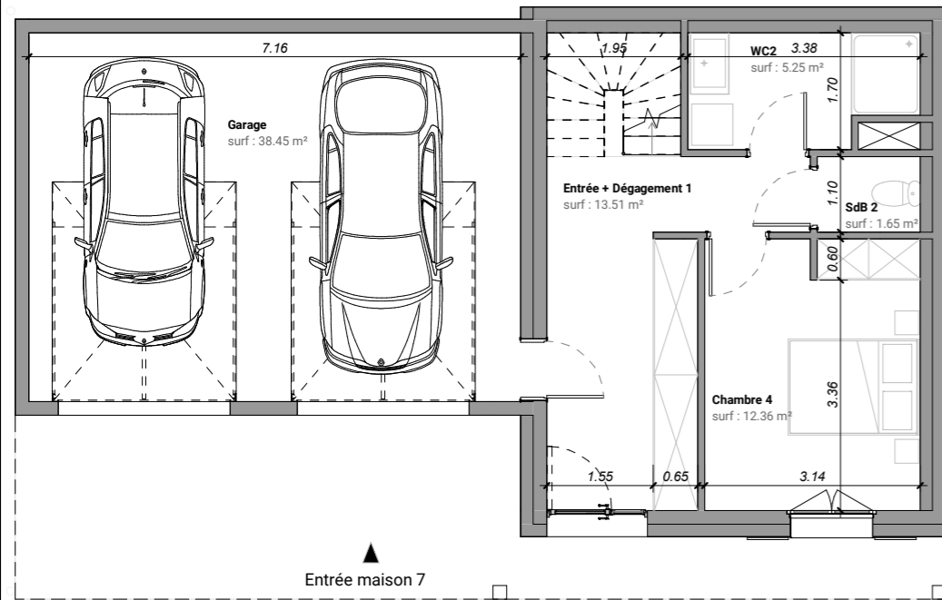
PLAN R-1
