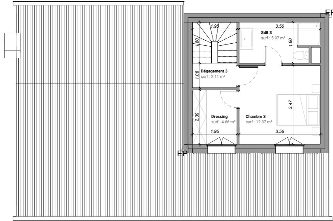
PLAN R+1
